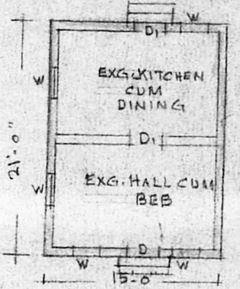
EXG. TILED HOUSE TO BE DEMOLISHED
