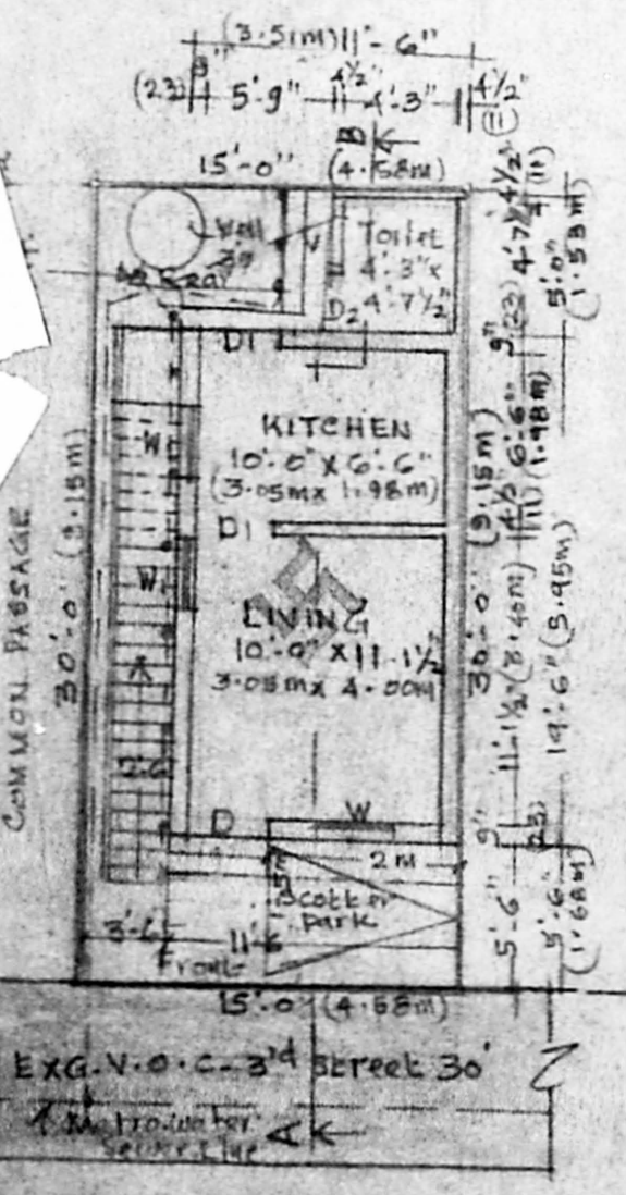
SITE & GR. FLOOR PLAN
